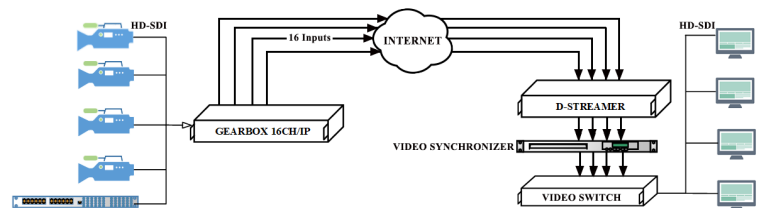
EXAMPLE VIDEO SYNCHRONIZER APPLICATION
